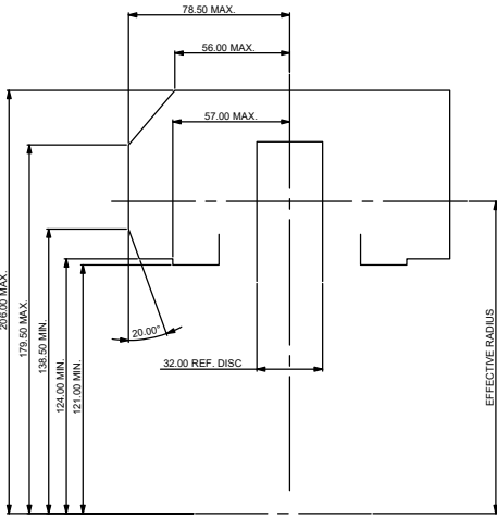
CALIPER RADIAL PROFILE AS FITTED ON Ø362.00 DISC.
